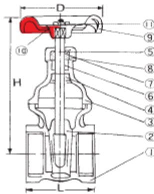
Figure BRGA – Bronze Gate Valve
