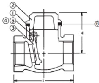
Figure BCH – Swing Check Valve
